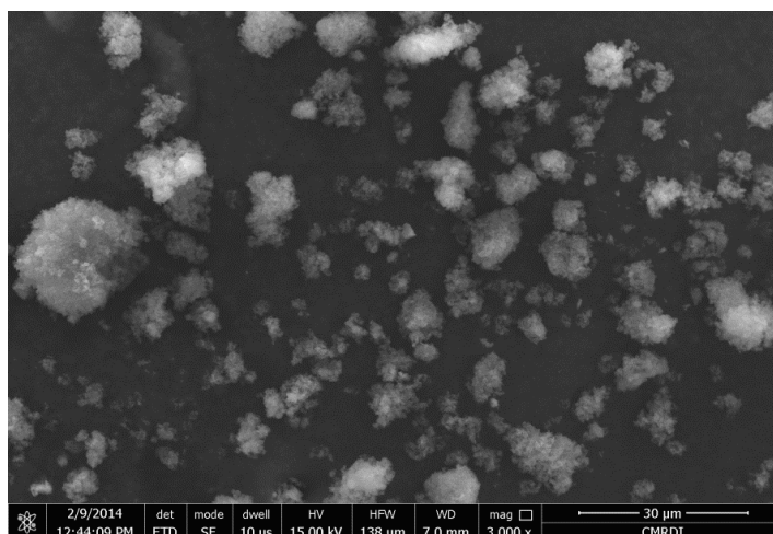
Figure 2: SEM micrograph of polyaniline (EB) powder.
