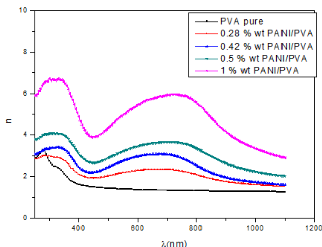
Fig (5) The refractive index of PANI/PVA blend at different concentration of PANI.
