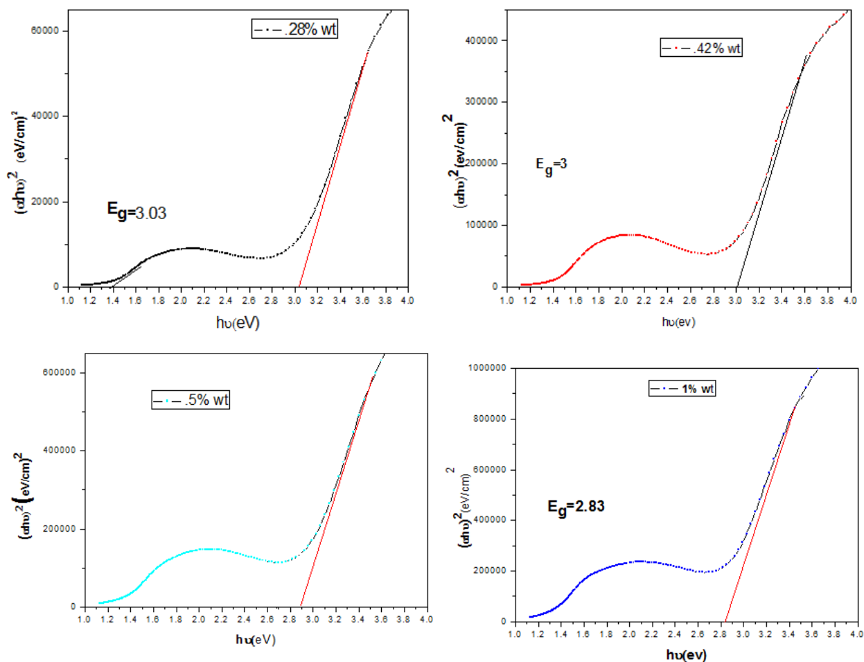
Fig(4) plots of (\alpha h\nu)^2 vs. (h\nu) for PANI/PVA blend films.
