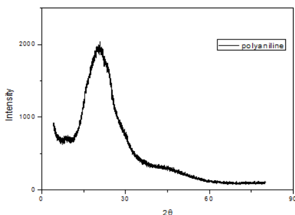
Fig. 1. XRD pattern of PANI powder.
