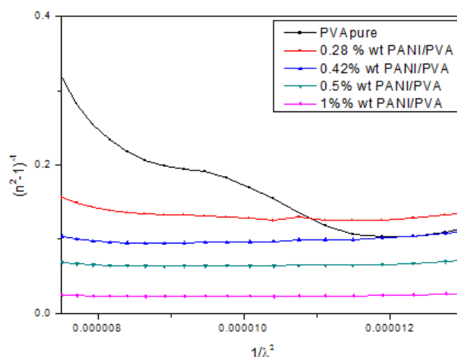
Fig (7) Plots of (a) (n^2-1)^{-1} vs. (h\omega)^2 (b) (n^2-1)^{-1} vs. (1/\lambda^2) for pure PVA and PANI /PVA blends.
