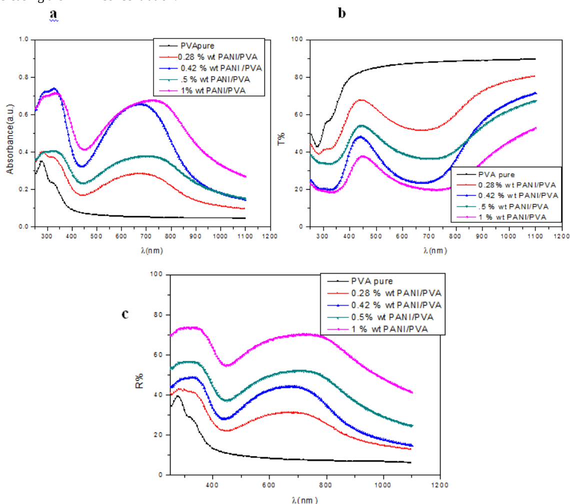
Fig (3) (a)Absorption, (b)transmission and (c)reflectance spectra as a function of wave length for PANI /PVA blend films.
