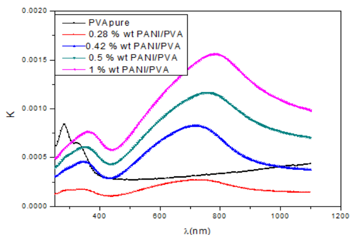
Fig (6) The extinction coefficient of PANI/PVA blend at different concentration of PANI.
