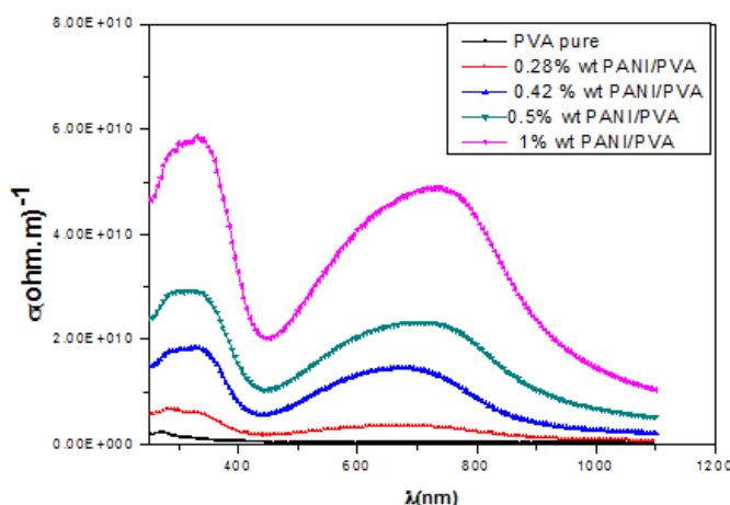
Fig (9) shows the variation of optical conductivity with wavelength for PVA pure and PANI/PVA blend.
